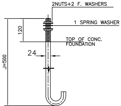
J-24x500 ANCHOR BOLT L-TYPE
