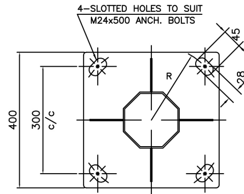
BASE PLATE DETAIL SIZE: 400x400x15 THK. 4 STIFFNER; SIZE: 70x70x10 THK.
