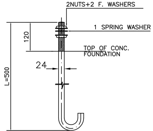
J-24x500 ANCHOR BOLT J-TYPE
