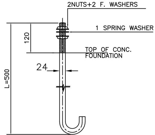
M24x500 ANCHOR BOLT J-TYPE
