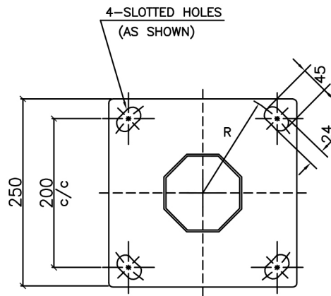
BASE PLATE DETAIL SIZE: 250x250x10 THK.
