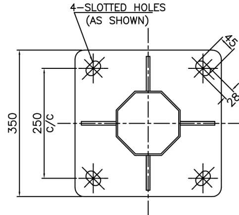
BASE PLATE DETAIL SIZE: 350x350x10 THK. 4 STIFFNER; SIZE: 70x70x10 THK.
