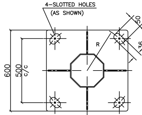
BASE PLATE DETAIL SIZE: 600x600x25 THK. 4STIFFNERS, SIZE: 120x75x10 THK.
