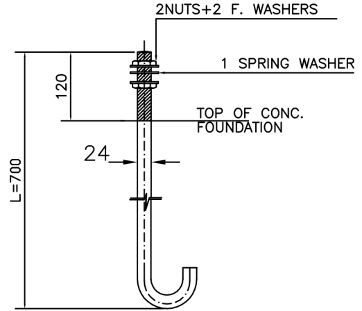
J-24x700 ANCHOR BOLT J-TYPE
