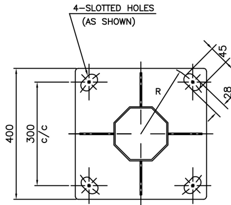
BASE PLATE DETAIL SIZE: 400x400x15 THK. 4 STIFFNER; SIZE: 70x70x10 THK.
