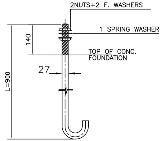
J-27x900 ANCHOR BOLT J-TYPE
