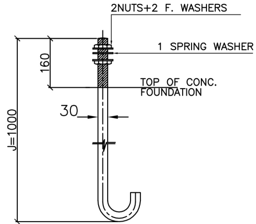
ANCHOR BOLT- J TYPE
