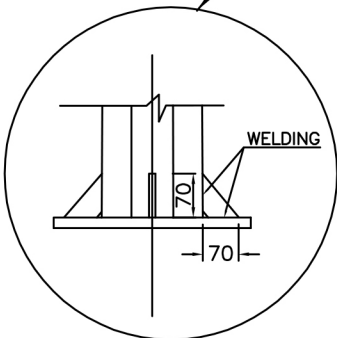
STIFFNER'S DETAILS
