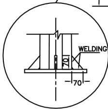
STIFFNER'S DETAILS
