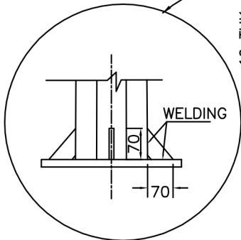
STIFFNER'S DETAILS
