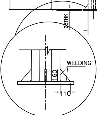
STIFFNER'S DETAILS
