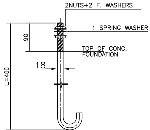
J-18x400 ANCHOR BOLT J-TYPE
