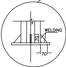
STIFFNER'S DETAILS
