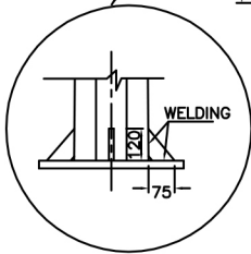
STIFFNER'S DETAILS
