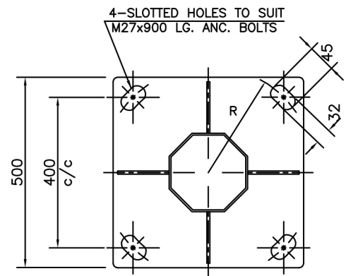
BASE PLATE DETAIL SIZE: 500x500x20 THK. 4STIFFNER, SIZE: 120x75x10 THK.
