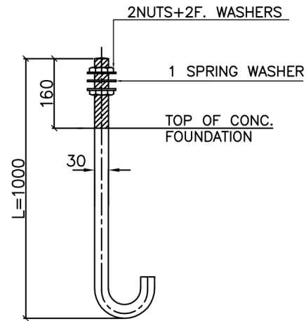
ANCHOR BOLT- J 30X1000
