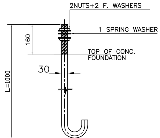
J-30x1000 ANCHOR BOLT J-TYPE
